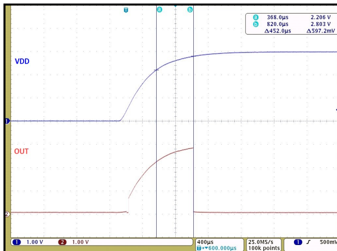
Figure 2. Power-On Time for Push-pull Output ( V_{DD} and \overline{\text{OUT}} )
